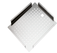
Tray, SS Perforated, 365 x 425 O.D 20.9236.SA
